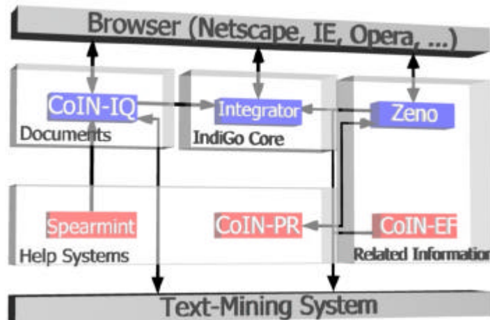
Fig. 2. Information flow in the indiGo platform
